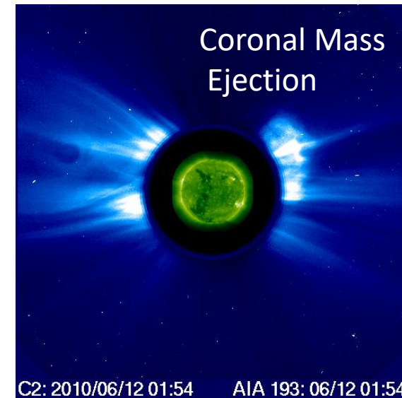
SOHO/SDO Image
