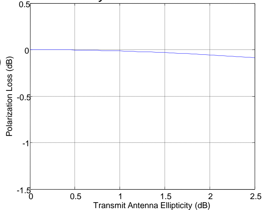
Polarization Loss at Worst Orientation into 0 dBic Circularly Polarized Receive Antenna
