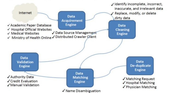
Figure 4. Data preprocessing workflow in the key opinion leader identification system.
