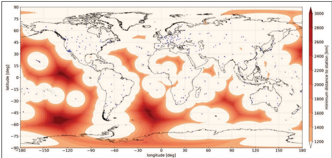
Figure 1: Global ionospheric coverage (see Key Point B) provided by the 515 stations currently available through the International GNSS Service network (see https://network.igs.org/ ). Some significant land areas are devoid of IGS stations, and could immediately benefit from additions to the network: e.g. , Africa, Indonesia, middle China, or Siberia. Coverage of the ocean is intrinsically more difficult; on certain islands, additional stations could however be added to the IGS network to fill critical gaps: e.g. , on the Kuna Atoll (United States) to cover the North-western Pacific Ocean, on Tristan da Cunha and the Falkland Islands (British Overseas Territories) to cover most of the Southern Atlantic Ocean, on Île Amsterdam (French Southern and Antarctic Lands) to decrease gaps over the Indian Ocean, etc. .
