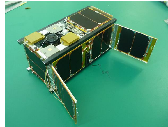
2U CubeSat RAIKO © Tohoku University
