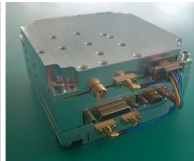
CubeSat S-band RF Transmitter and Receiver, X-band Transmitter, and inside of the X-band Transmitter (from left to right) © Addnics corp.
