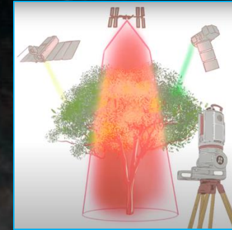
Estimating Above Ground Biomass with Lidar
